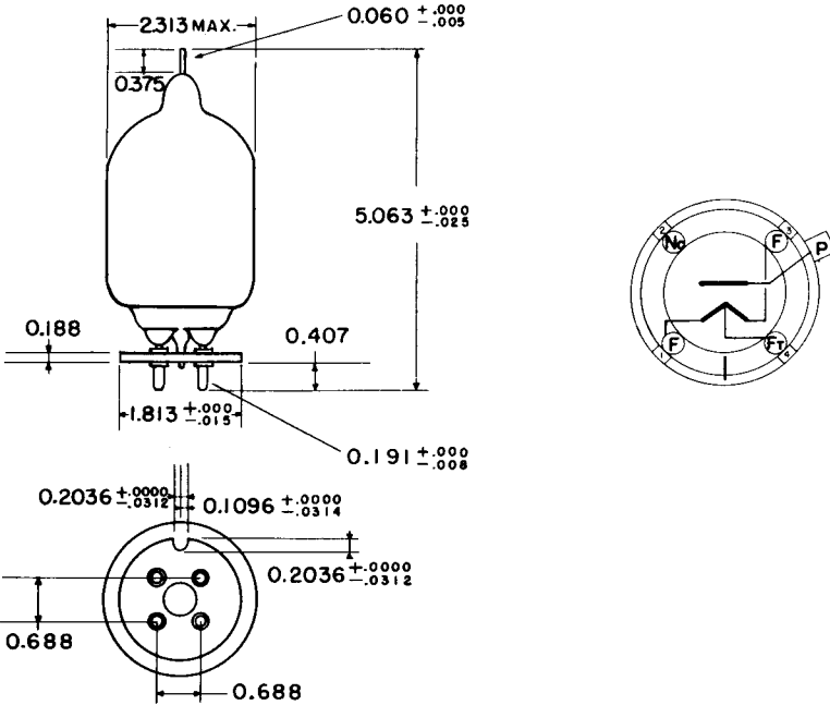
TUBE DIMENSIONS
